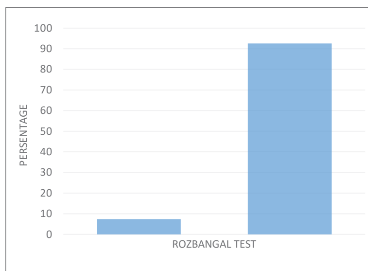
Figure 2. Percentage frequency of the Rose Bengal test result in the studied samples
