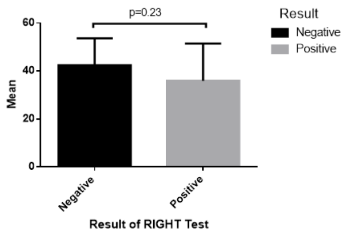
Figure 3. Comparison of the mean age in the two groups with negative and positive Wright test results
