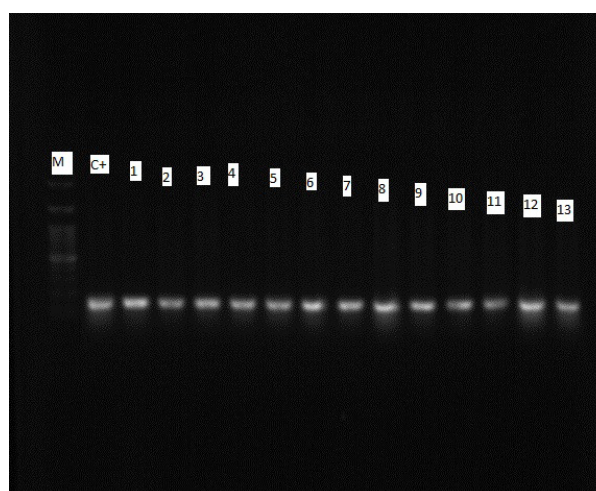
Figure 1. Agarose gel electrophoresis of the AmpC gene of clinical Kp isolates Lanes 1-13: Kp carrying the AmpC gene (190bp), C+: E. coli ATCC 25922, M: 100 bp DNA ladder.
